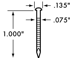
Item Number: BGN-15 Description: 1" Bright Galvanized Round Head Nail Material: Steel
