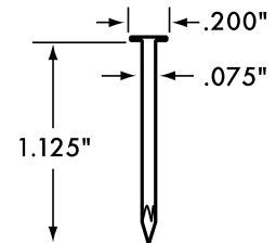
Item Number: GN-3D Description: 1.125" Galvanized Flat Head Nail Material: Steel
