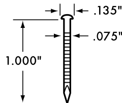
Item Number: BGN-15 Description: 1" Bright Galvanized Round Head Nail Material: Steel
