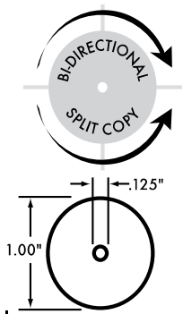
Item Number: BD1-18 Description: 1" Date Disc .125" Dia. Hole Material: Bronze
