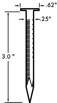
Item Number: BDN-3 Description: 3" Date Nail Material: Bronze
