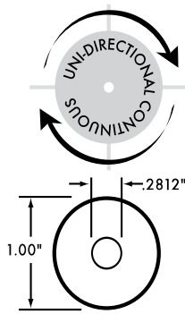
Item Number: AD1-932 Description: 1" Date Disc .2812" Dia. Hole Material: Aluminum
