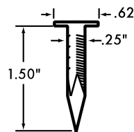
Item Number: AD Description: 1.5" Date Nail Material: Aluminum
